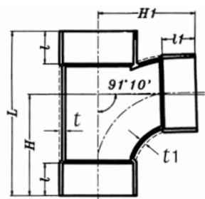
順T型同徑接頭 Sanitary Tee
